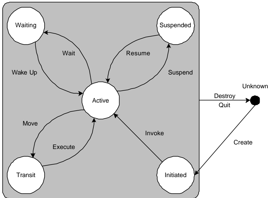
Figure 3 - Agent life-cycle as defined by FIPA.
