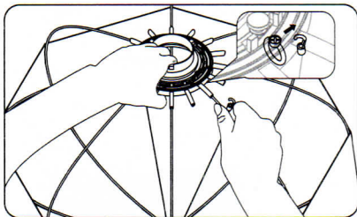
9. Remove the hook from both sides of the fixing ring.
