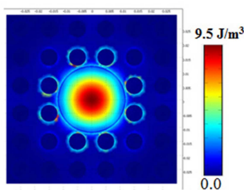
Figures : a) Numerical simulation of the strain energy density confinement by an AM from an acoustic sound pressure of 1Pa. b) An example of acoustic metamaterial for energy harvesting.
