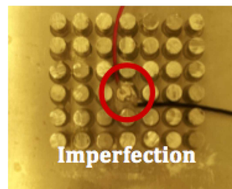
Figures : a) Numerical simulation of the strain energy density confinement by an AM from an acoustic sound pressure of 1Pa. b) An example of acoustic metamaterial for energy harvesting.
