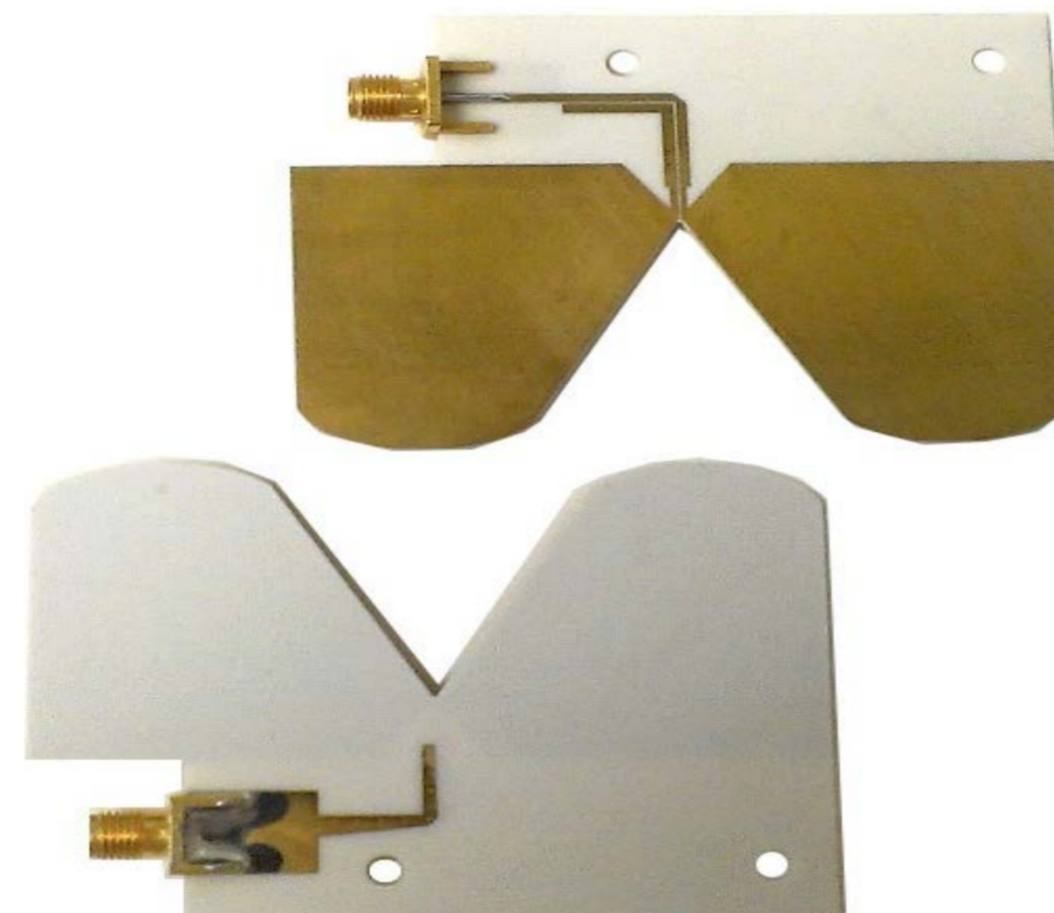
Bow-tie antenna
