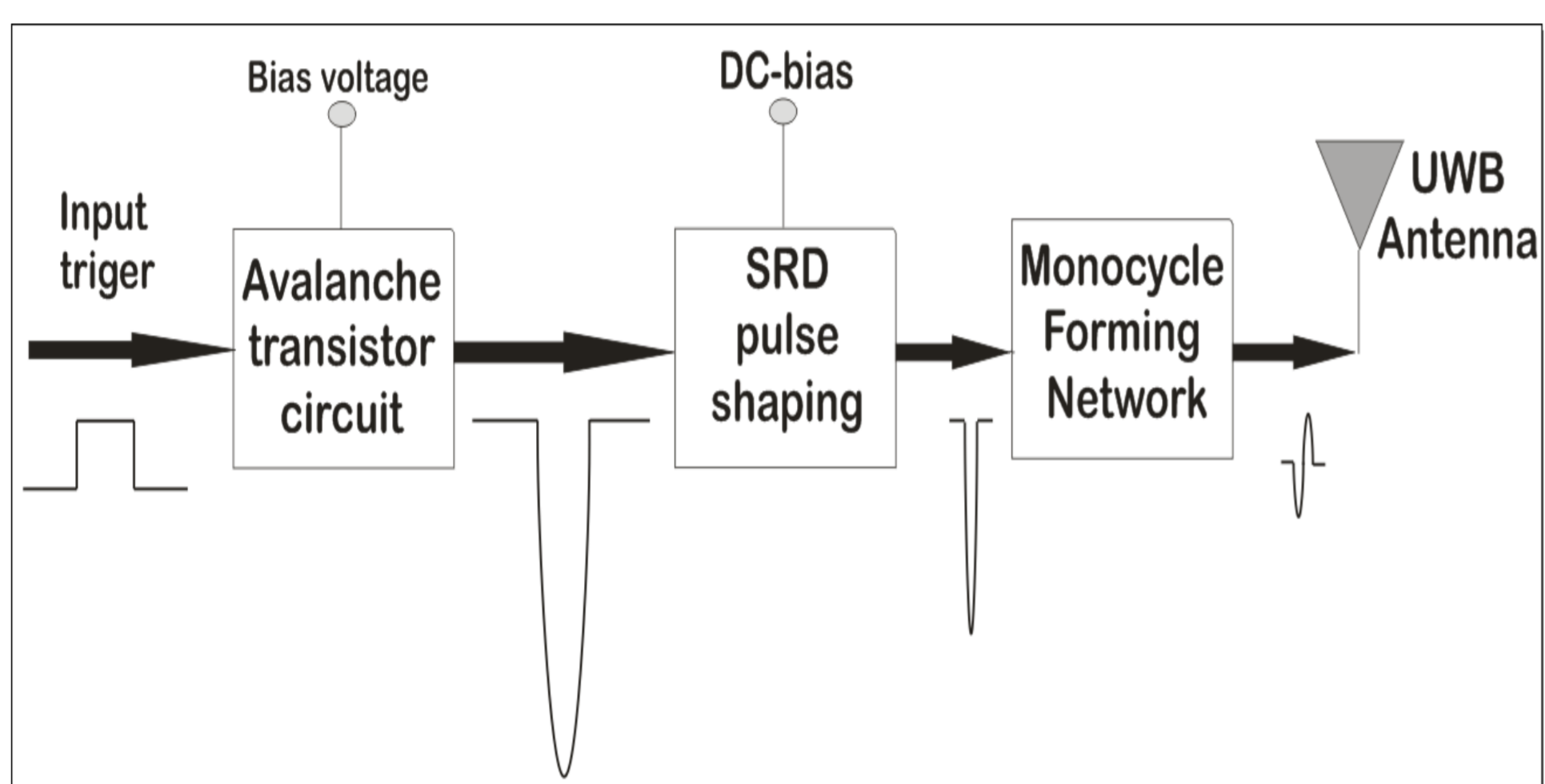
Designed Circuit Propose
